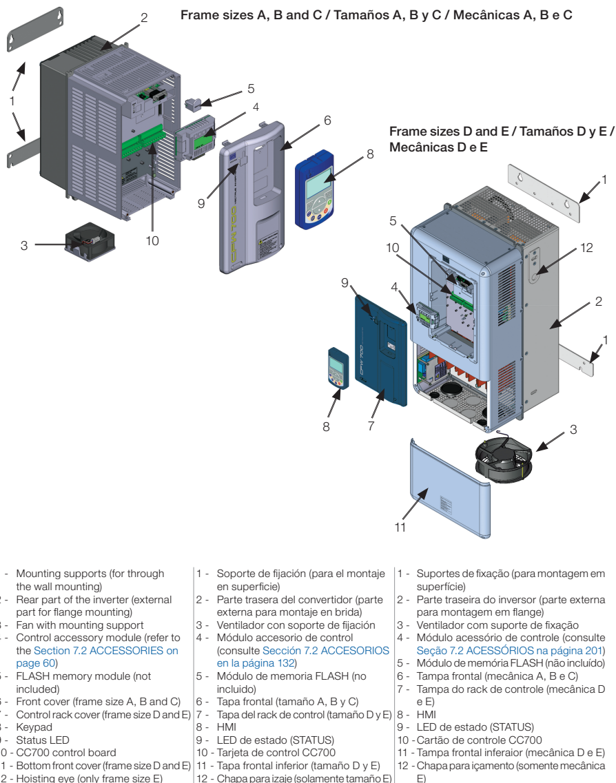
Figure A.1: Main components of the CFW700
