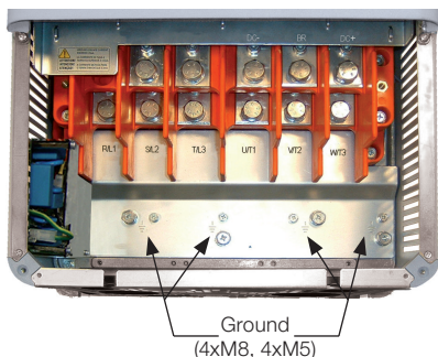
(e) Frame size E
