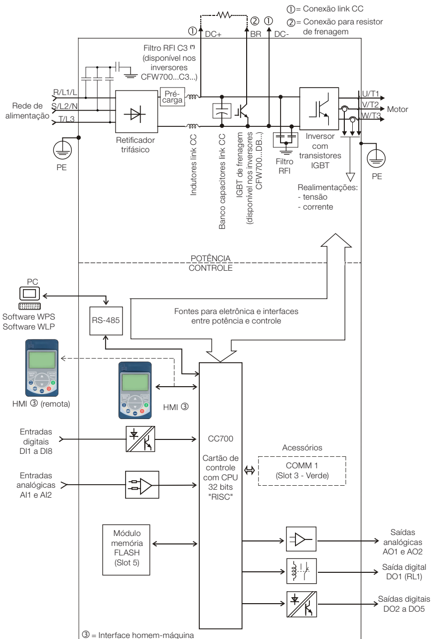
Figura 2.1: Blocodograma do CFW700
