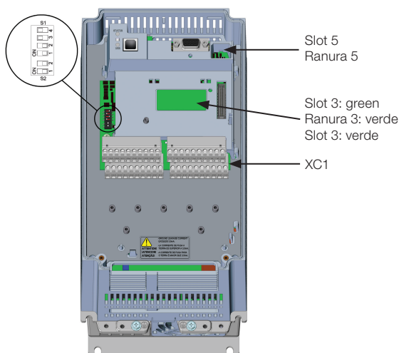
Figure A.3: Location of the control board, XC1 terminal strip (control signals), and S1 (analog inputs and outputs signal type selection) and S2 (RS-485 line termination) DIP-switches
