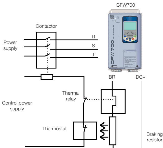
Figure 3.3: Connection of the braking resistor
