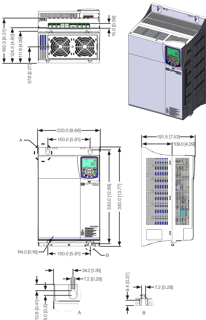
Figure B.8: Inverter dimensions in mm [in] – frame size E
