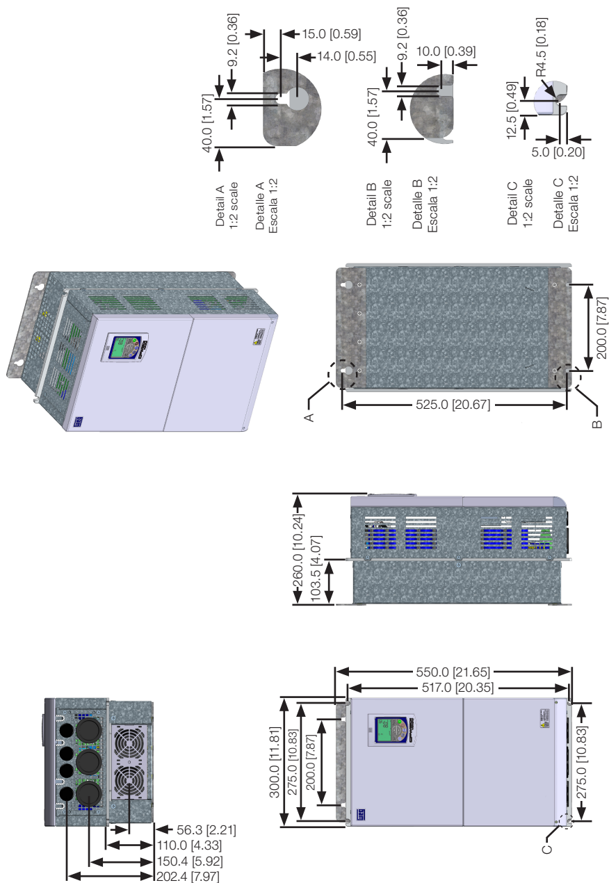
Figure B.9: Inverter dimensions in mm [in] – frame size F
