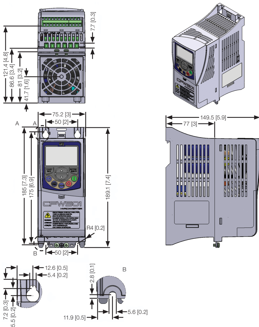
Figure B.4: Inverter dimensions in mm [in] – frame size A
