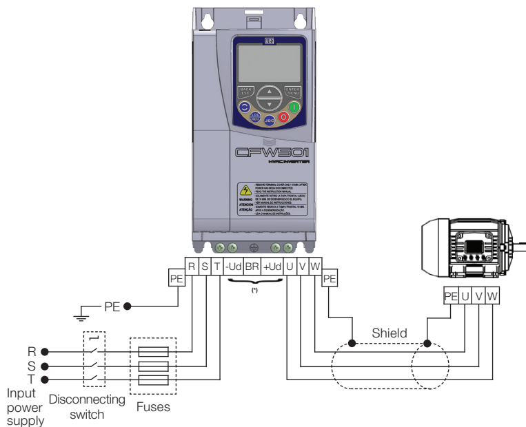
(a) Frame sizes A, B, C and F
