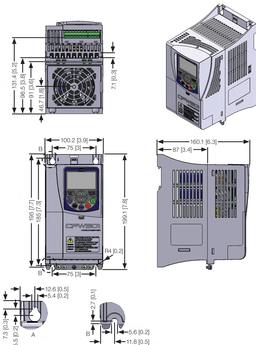
Figure B.5: Inverter dimensions in mm [in] – frame size B
