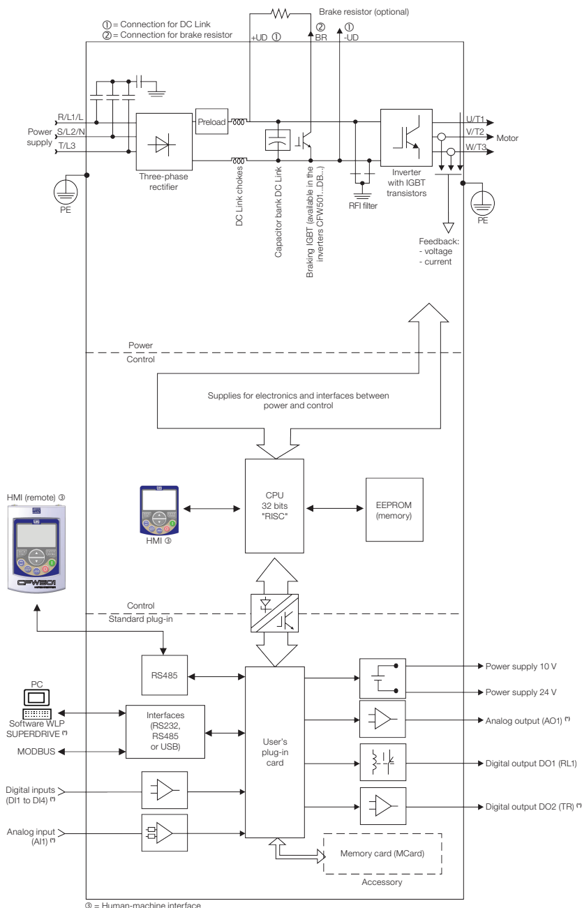
Figure 2.3: Block diagram of CFW501 for frame sizes F and G
