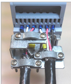
Figure 3.3: Details of the connection of the power supply and the motor cable shield to the accessory CFW500-KPCSA
