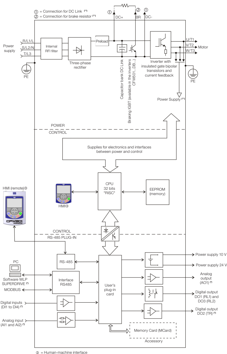
Figure 2.1: Block diagram of CFW501 for Frame sizes A, B and C
