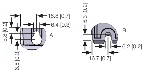
Figure B.6: Inverter dimensions in mm [in] – frame size C
