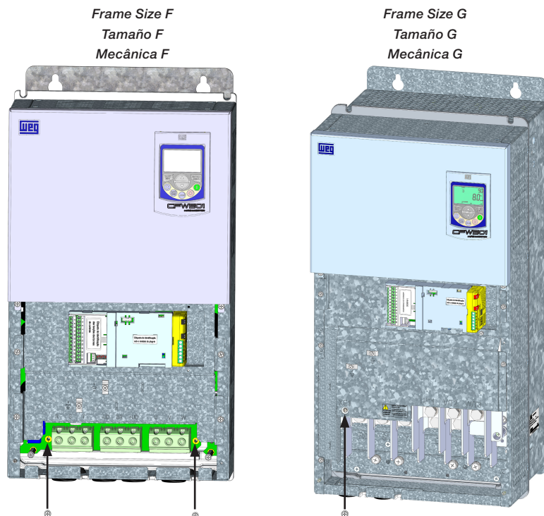
Figure A.4: Location of filter capacitors ground disconnection points - disconnection trough bolts - frame sizes F and G
