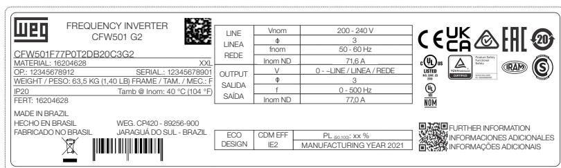
(b) Side label of the CFW501 - frame sizes F and G
