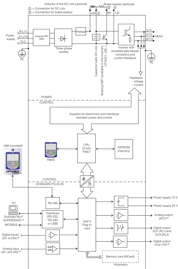
Figure 2.2: Block diagram of CFW501 for Frame sizes D and E
