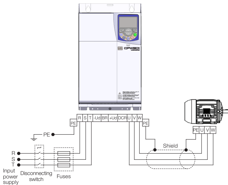
(b) Frame sizes D and E
