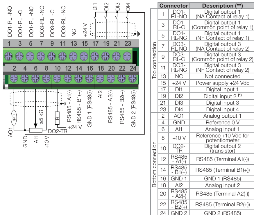
Figure 3.4: Signals of the connector of the CFW500-CRS485-B plug-in module
