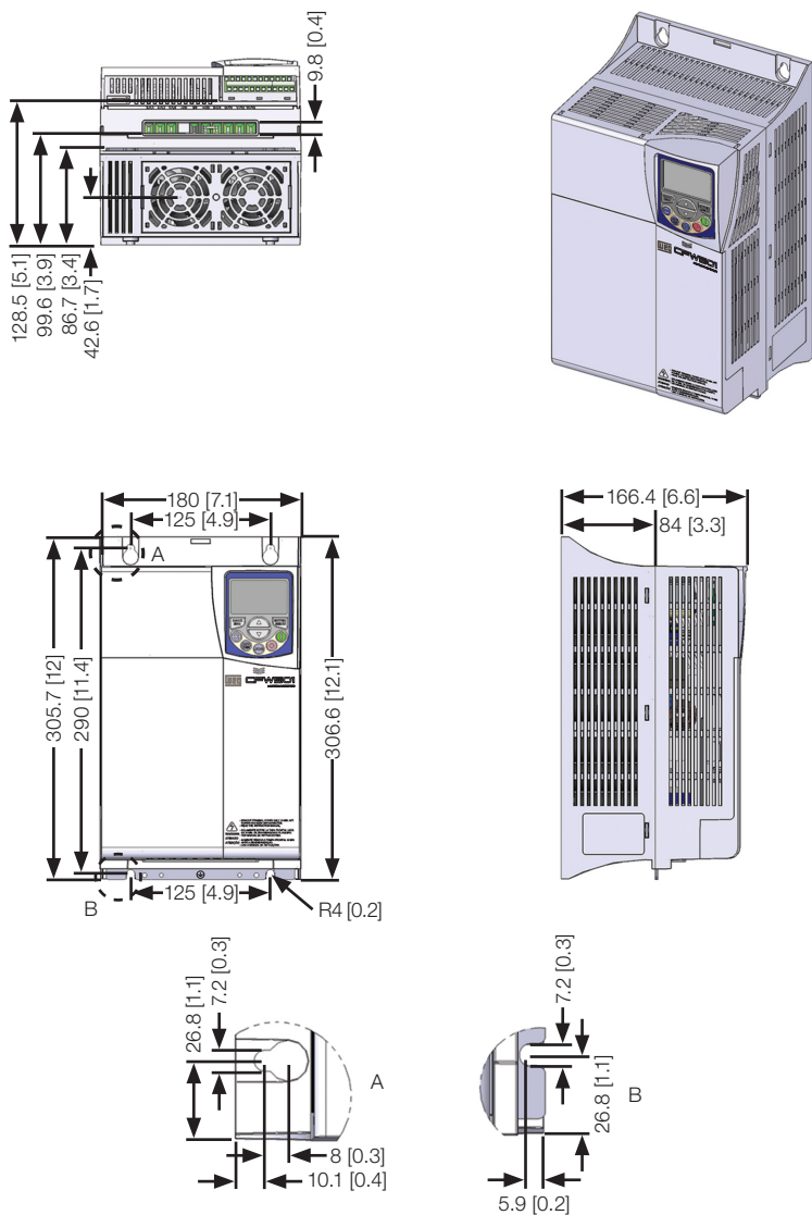
Figure B.7: Inverter dimensions in mm [in] – frame size D
