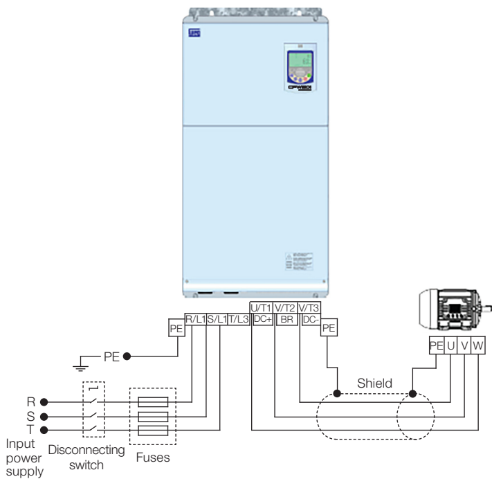
(c) Frame size G
