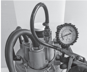
Fig. 2 Applying 2kg/cm2 air pressure.
