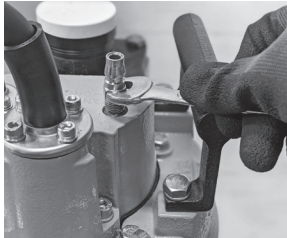
Fig. 1 Quick Coupler Installation.
