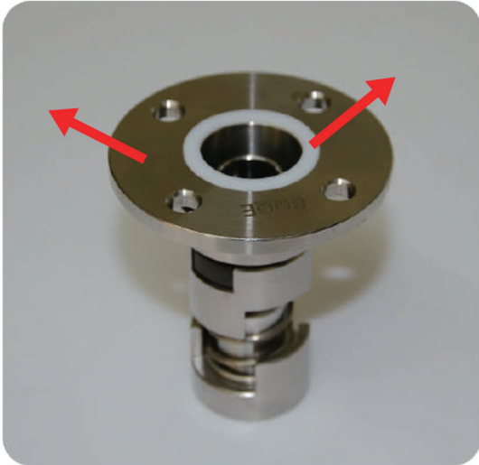
Step3: take the gasket out and remove the set base of shaft sea
